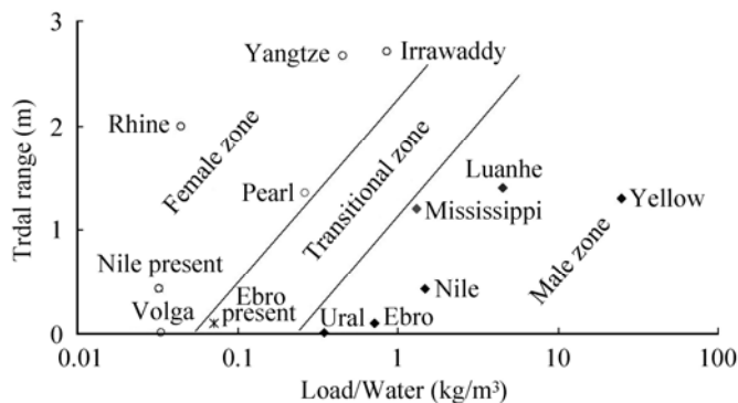
Fig. 8 Gender of the delta as a function of sediment load/water ratio and tidal range
