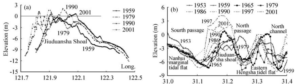
Fig. 6 Development of the Jiuduansha Shoal: (a) Longitudinal section of the Jiuduansha Shoal (121°35'E, 31°16'N-122°25'E, 31°5'N, Figure 5 as A-A') from 1959 to 2001; (b) Cross section of the Jiuduansha Shoal at 122°E (Figure 5 as B-B') from 1953 to 2001
