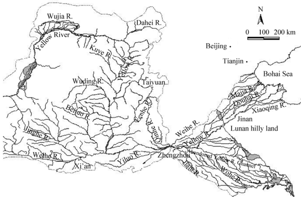
Fig. 11 The Yellow River and its parasitizing rivers
