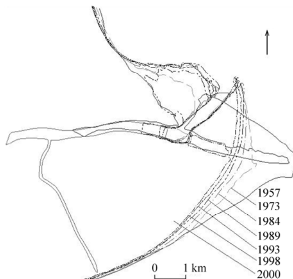
Fig. 10 Retreating Ebro delta due to sharp reduction in sediment load in the past 50 years (after Ibáñez and Rovira, 2009)
