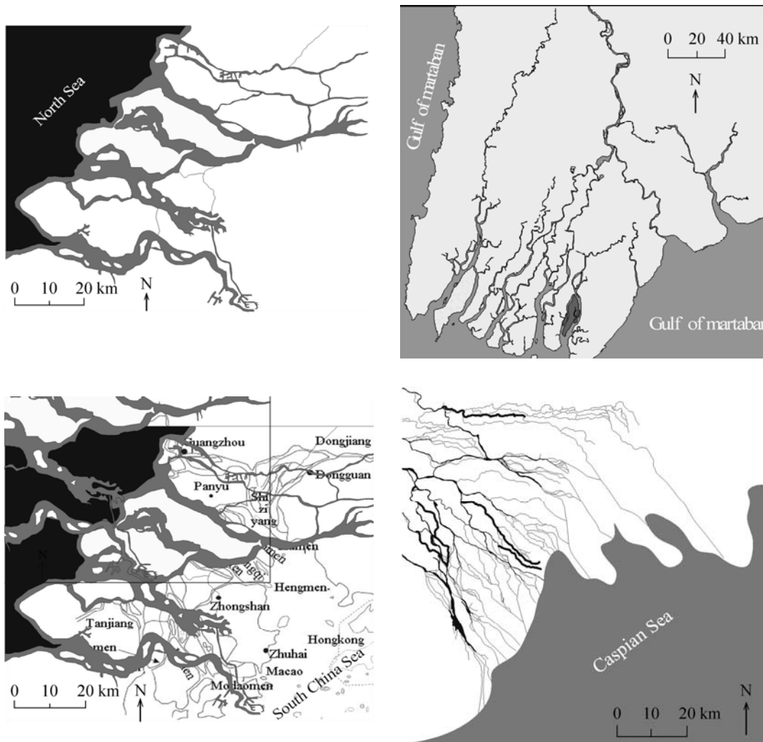
(a) Rhine-Meuse-Scheldt delta; (b) Irrawady delta; (c) Pearl River delta; and (d) Volga delta Fig. 7 Female deltas consist of numerous islands and spider-web like channels:
