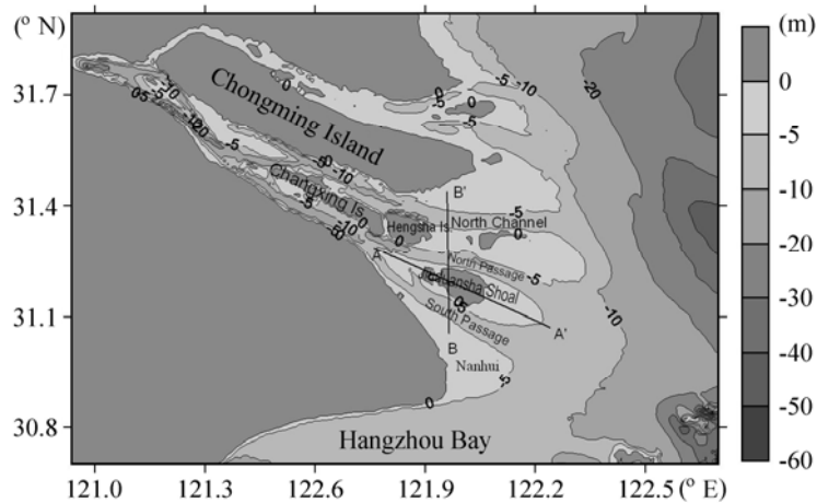
Fig. 5 The Yangtze River delta - Chongming Island divides the river into the North and South Branches; Changxing Island divides the South Branch into the North and South Channels; and Jiuduansha Shoal divides the South Channel into the North and South Passages
