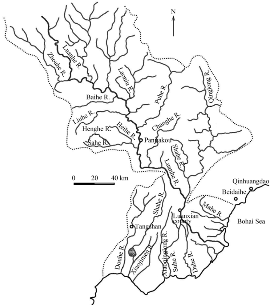
Fig. 12 The Luanhe River and its parasitizing rivers
