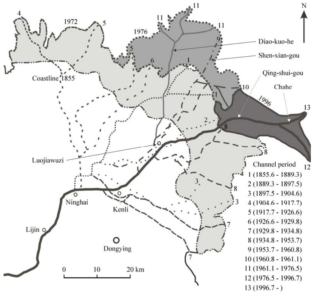
Fig. 2 Nodal avulsions and the abandoned channels on the present Yellow River delta
