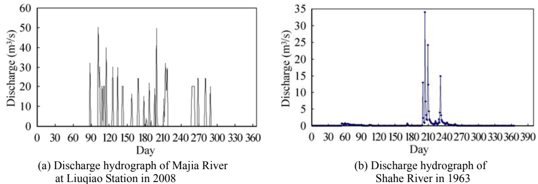
Fig. 13 Sharp peaks of discharge during the rain season of parasitizing rivers: (a) Majia River- a parasitizing river of the Yellow River; (b) Shahe River- a parasitizing river of the Luanhe River
