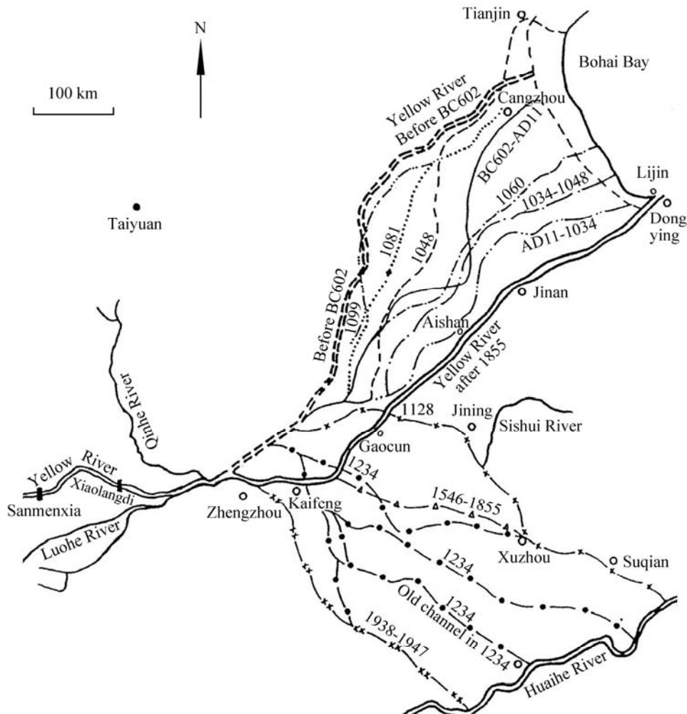
Fig. 1 Migration of the lower Yellow River and old channels due to avulsions in the past 2600 years
